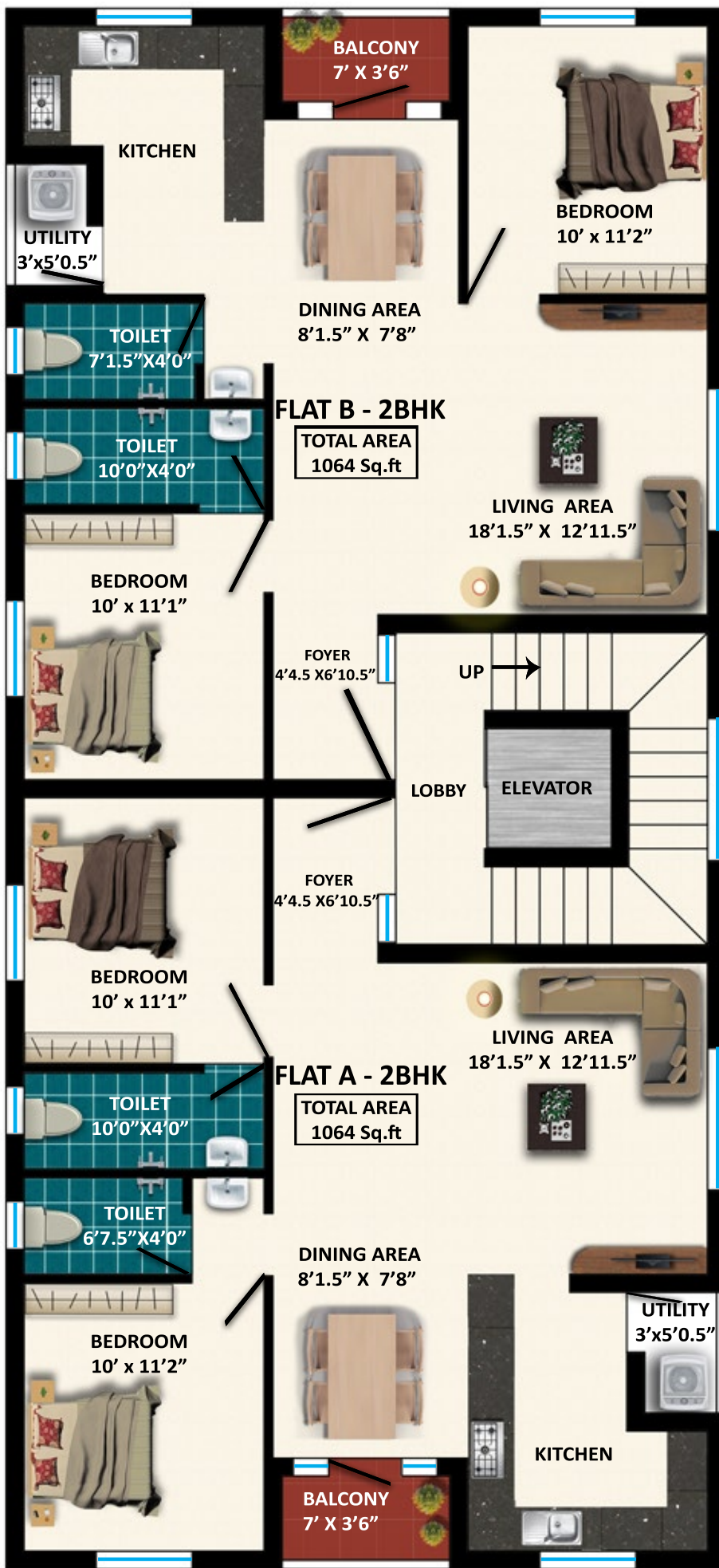
BLOCK B - TYPICAL FLOOR PLAN (Floors 1-3) SAI SUBASHYA - SUSEELA TOWERS
